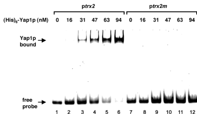
FIGURE 3: Characterization of in vitro purified (His) 6 -Yap1p. Binding of (His) 6 -Yap1p to the TRX2 promoter was assayed by incubating increasing concentrations of purified oxidized Yap1p with 5'-FAM labeled ptrx2 (lanes 1–6) or ptrx2m (lanes 7–12).
