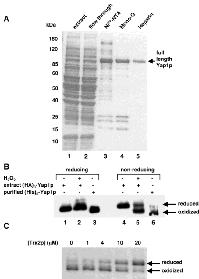
FIGURE 2: Oxidation and reduction of in vitro purified (His) 6 -Yap1p. (A) Coomassie blue stained SDS-PAGE gel of the purification of (His) 6 -Yap1p from S. cerevisiae . Lanes: 1, crude yeast extract; 2, flow through from the Ni 2+ -NTA column; 3, 150 mM imidazole fraction from the Ni 2+ -NTA column; 4, Mono Q (His) 6 -Yap1p fraction; 5, Hi-trap Heparin (His) 6 -Yap1p fraction. (B) Western blot of in vivo (HA) 3 -Yap1p and in vitro purified (His) 6 -Yap1p separated on reducing (lanes 1–3) and nonreducing (lanes 4–6) SDS-PAGE gels. Lanes: 1, (HA) 3 -Yap1p untreated; 2, (HA) 3 -Yap1p + H 2 O 2 ; 3, (His) 6 -Yap1p; 4, (HA) 3 -Yap1p untreated; 5, (HA) 3 -Yap1p + H 2 O 2 ; 6, (His) 6 -Yap1p. (C) Incubation of (His) 6 -Yap1p with increasing concentrations of Trx2p.
