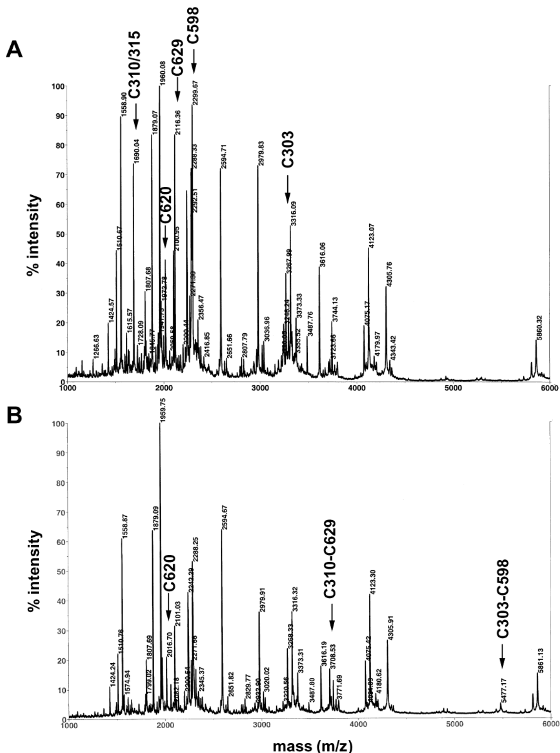
FIGURE 4: MALDI-TOF MS of reduced (A) and oxidized (B) (His) 6 -Yap1p. Oxidized (His) 6 -Yap1p was digested overnight with endoproteinase Lys-C (Roche) in the presence of 10 mM IAA at 37 °C. Half of the sample was reduced with 10 mM DTT at 37 °C for 1 h. Cysteine-containing peptides are indicated with arrows.
